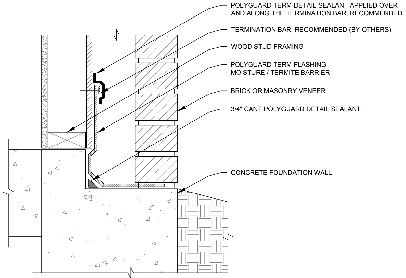
SECTION @ TERM © FLASHING / MOISTURE TERMITE BARRIER IN CAVITY WALL (FOR USE WHEN TERM © SILL / MOISTURE TERMITE BARRIER HAS NOT BEEN PREVIOUSLY INSTALLED)
